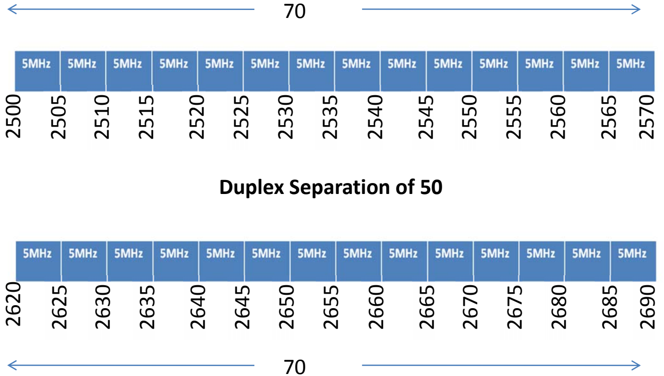
Figure 11: Frequency allocation for Spectrum in the 2.6 GHz band
