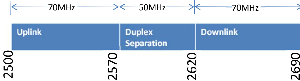
Figure 10: Nigerian Communications Commission frequency allocation map
